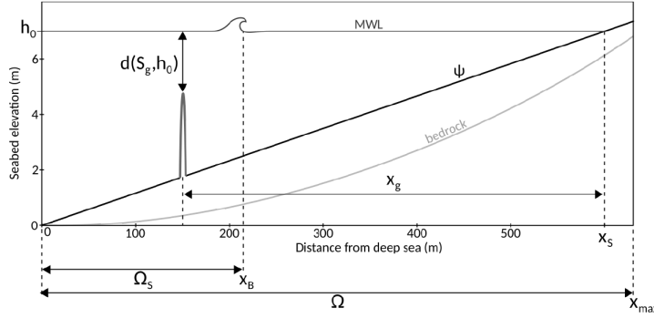
Figure 0.8 – Configuration of the geotube simulation.
