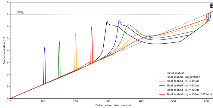
Figure 0.9 – Final seafloor profiles produced by the Opti-Morph morphodynamic model with variable geotube positions on the cross-shore profile.
